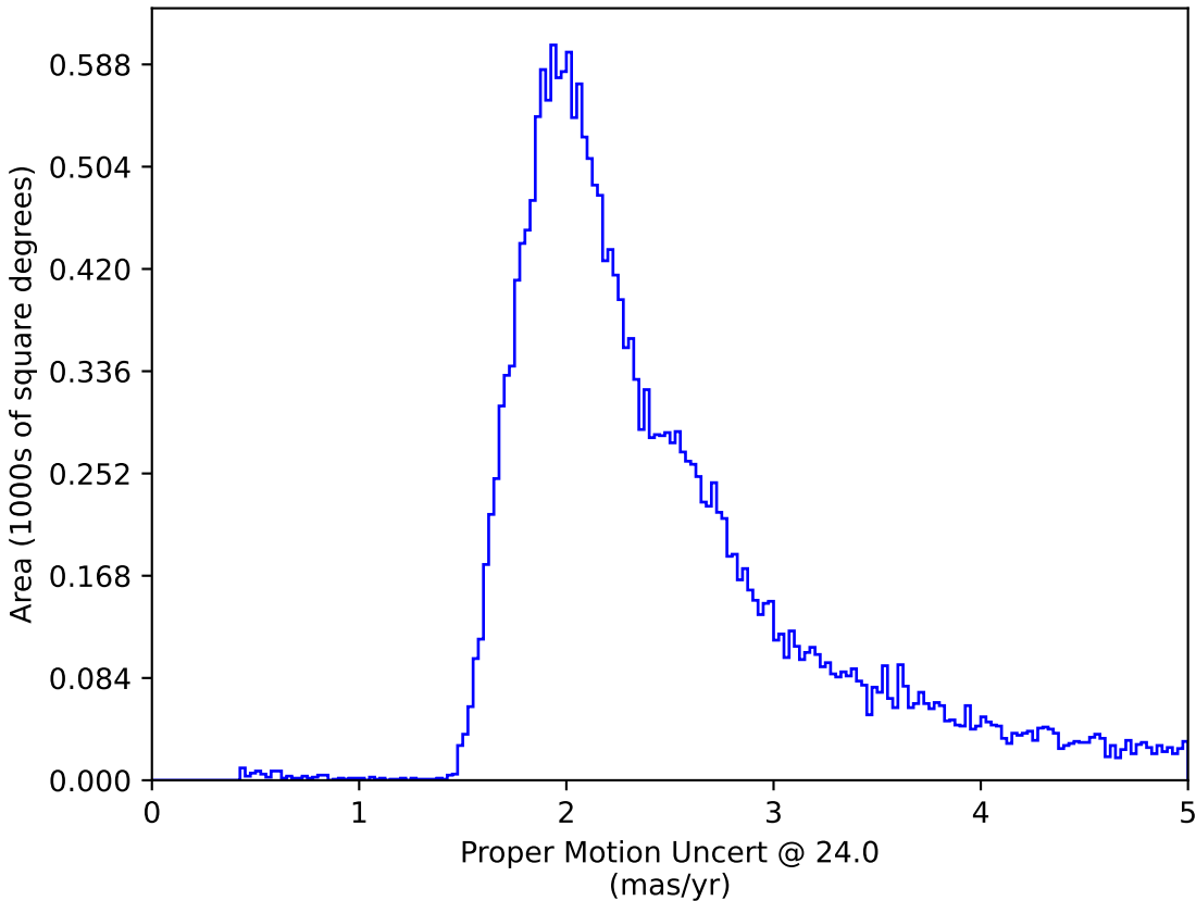
too_elab_r8_d2_ugrizy_v3.4_10yrs : Proper Motion Uncert @ 24.0
