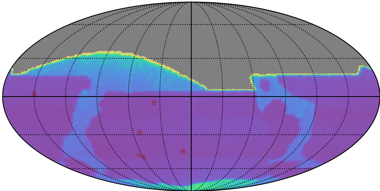
too_elab_r8_d2_ugrizy_v3.4_10yrs : Proper Motion Uncert @ 20.5
