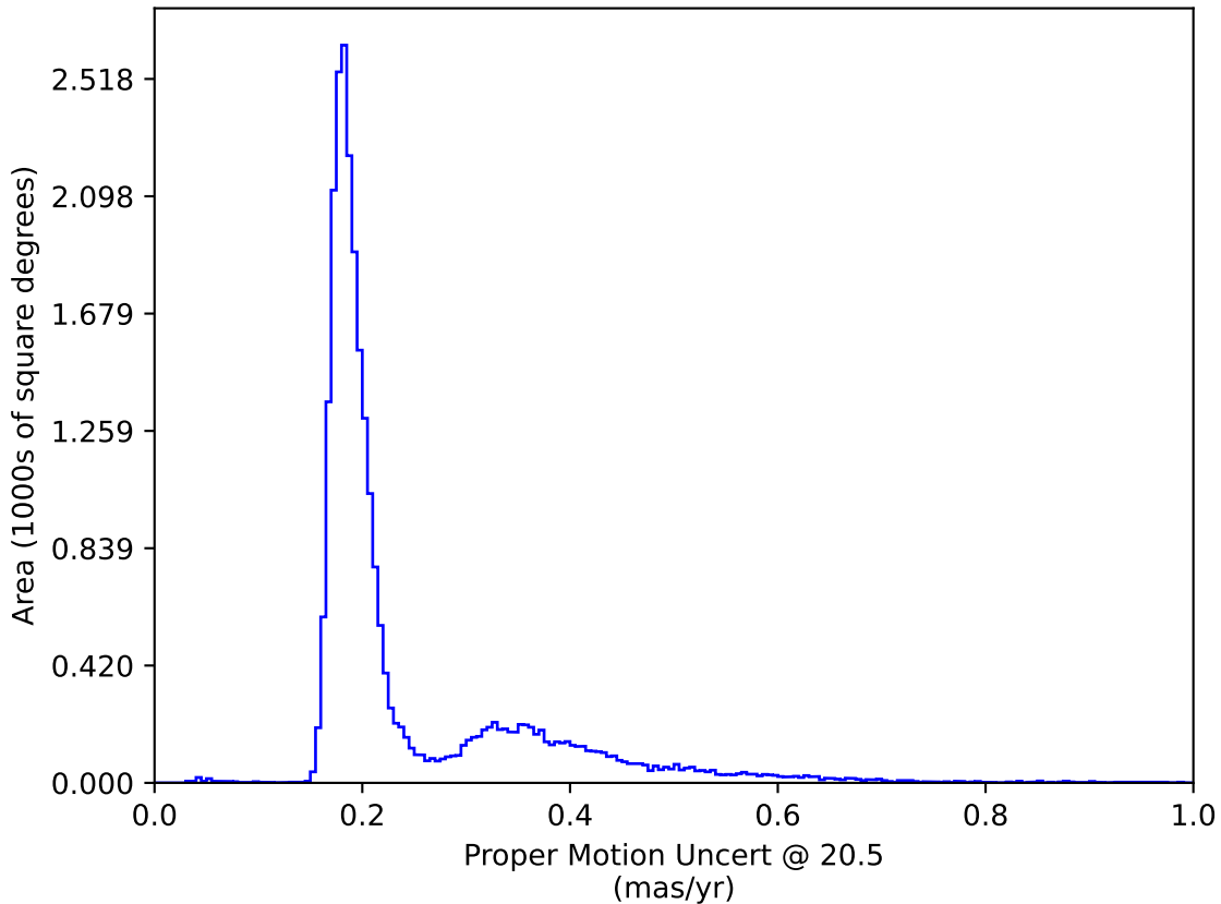
too_elab_r8_d2_ugrizy_v3.4_10yrs : Proper Motion Uncert @ 20.5
