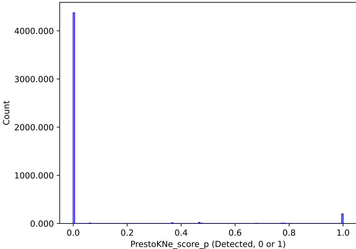
too_elab_r8_d2_ugrizy_v3.4_10yrs : PrestoKNe_score_p
