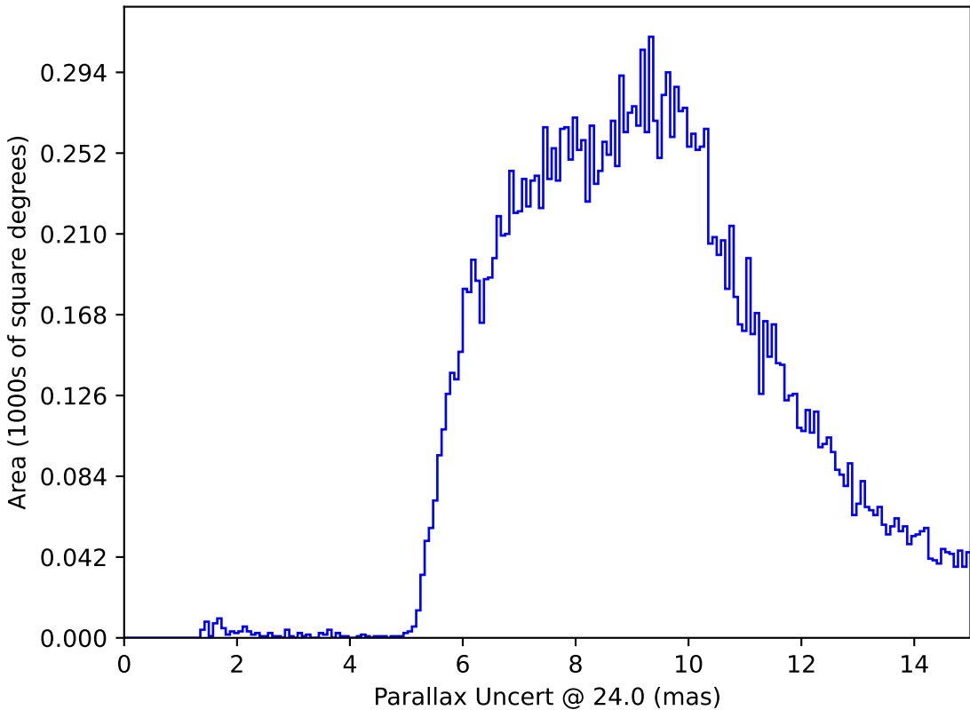
too_elab_r8_d2_ugrizy_v3.4_10yrs : Parallax Uncert @ 24.0
