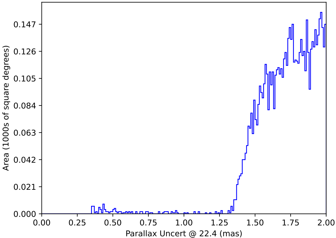
too_elab_r8_d2_ugrizy_v3.4_10yrs : Parallax Uncert @ 22.4
