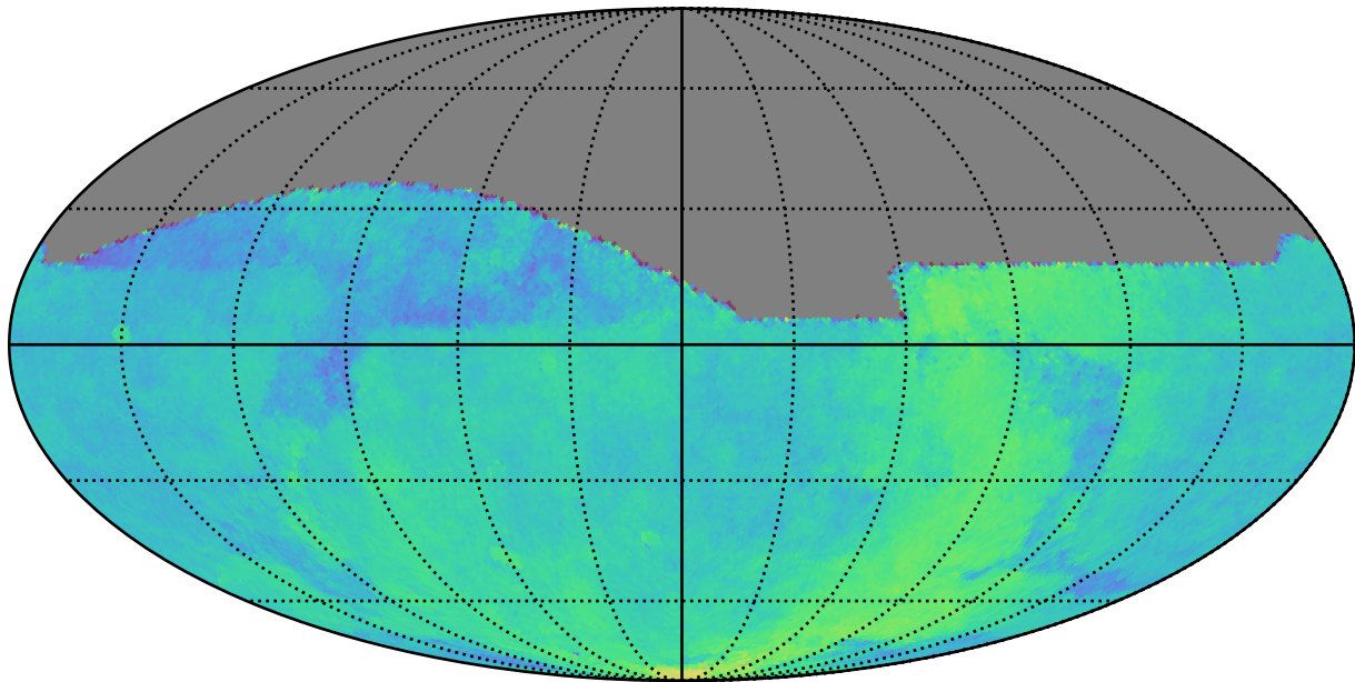
too_elab_r8_d2_ugrizy_v3.4_10yrs : Parallax Coverage @ 24.0
