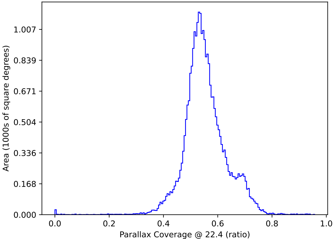
too_elab_r8_d2_ugrizy_v3.4_10yrs : Parallax Coverage @ 22.4
