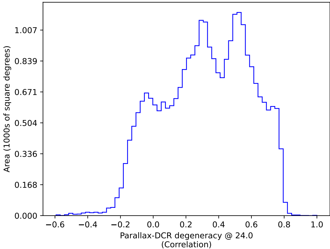
too_elab_r8_d2_ugrizy_v3.4_10yrs : Parallax-DCR degeneracy @ 24.0
