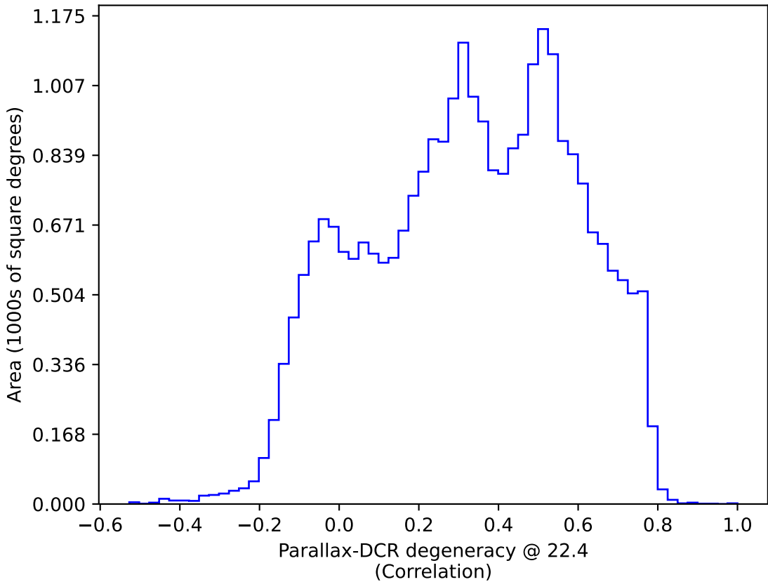
too_elab_r8_d2_ugrizy_v3.4_10yrs : Parallax-DCR degeneracy @ 22.4
