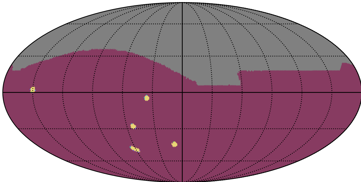
too_elab_r8_d2_ugrizy_v3.4_10yrs : NumberOfQuickRevisits
