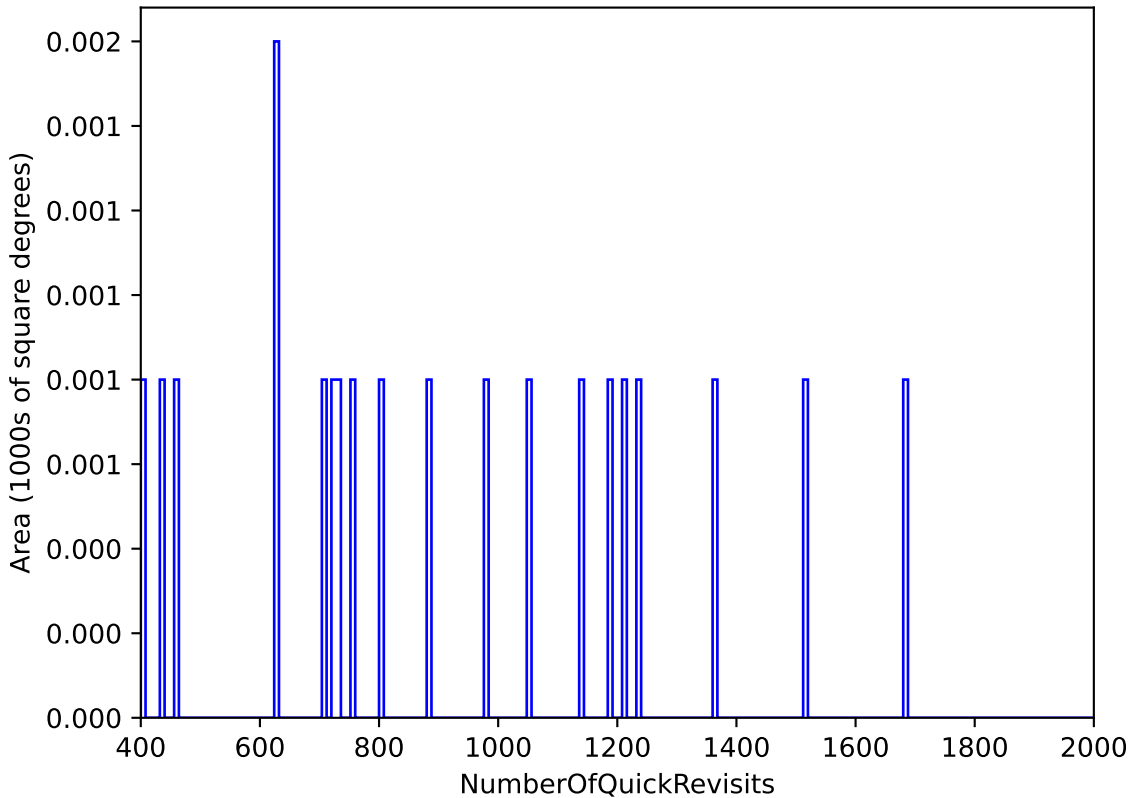
too_elab_r8_d2_ugrizy_v3.4_10yrs : NumberOfQuickRevisits
