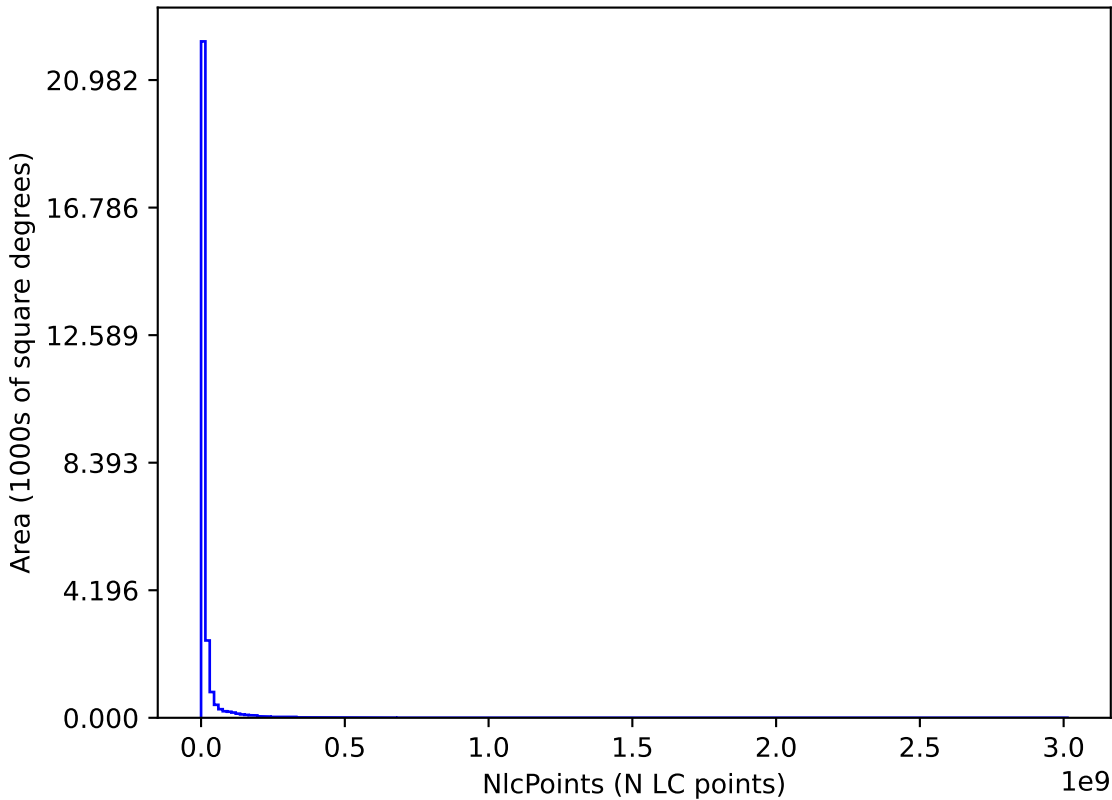
too_elab_r8_d2_ugrizy_v3.4_10yrs : NlcPoints
