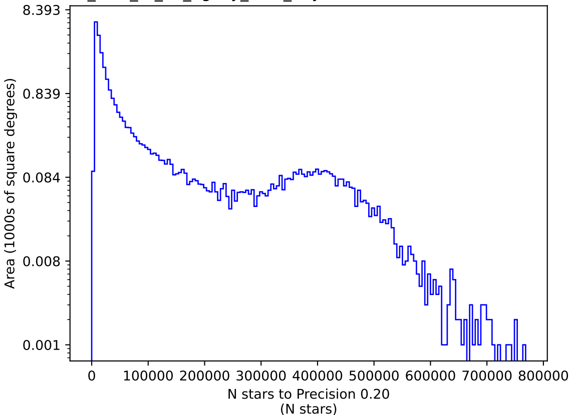
too_elab_r8_d2_ugrizy_v3.4_10yrs z: N stars to Precision 0.20
