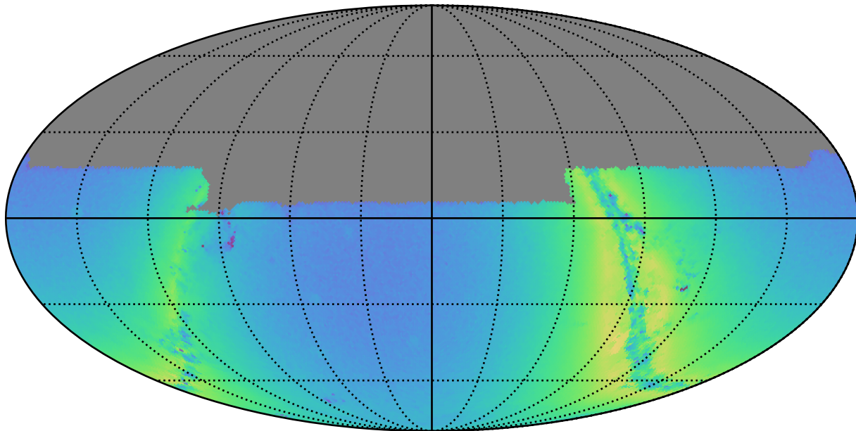
too_elab_r8_d2_ugrizy_v3.4_10yrs u: N stars to Precision 0.20
