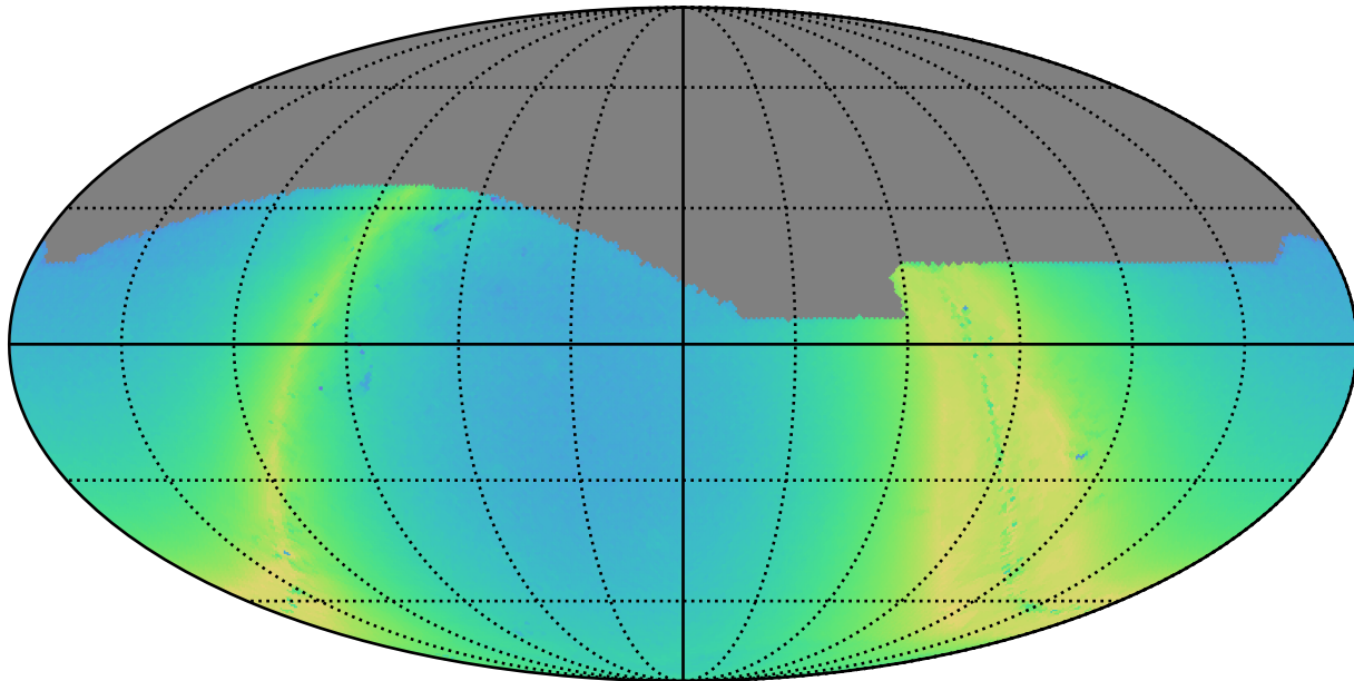
too_elab_r8_d2_ugrizy_v3.4_10yrs r: N stars to Precision 0.20
