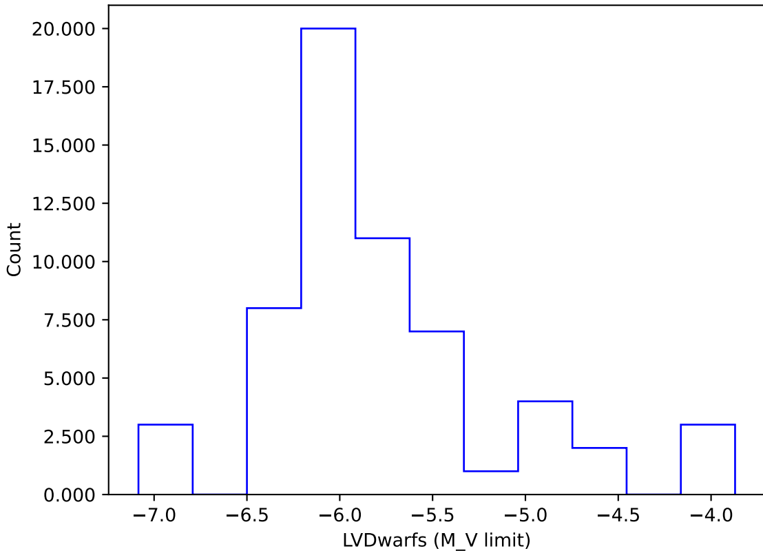
too_elab_r8_d2_ugrizy_v3.4_10yrs gi: LVDwarfs
