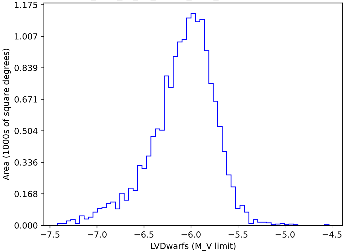
too_elab_r8_d2_ugrizy_v3.4_10yrs gi: LVDwarfs
