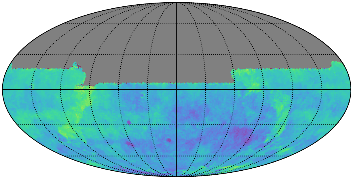
too_elab_r8_d2_ugrizy_v3.4_10yrs y: Kuiper rotSkyPos
