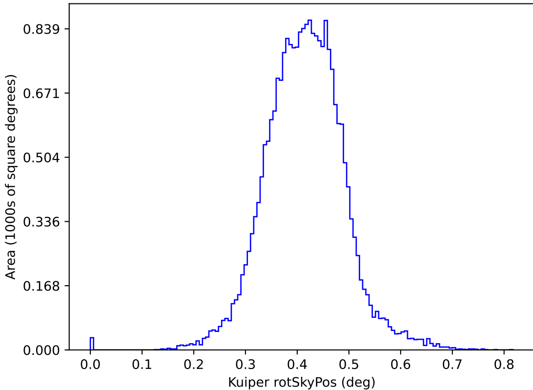
too_elab_r8_d2_ugrizy_v3.4_10yrs y: Kuiper rotSkyPos
