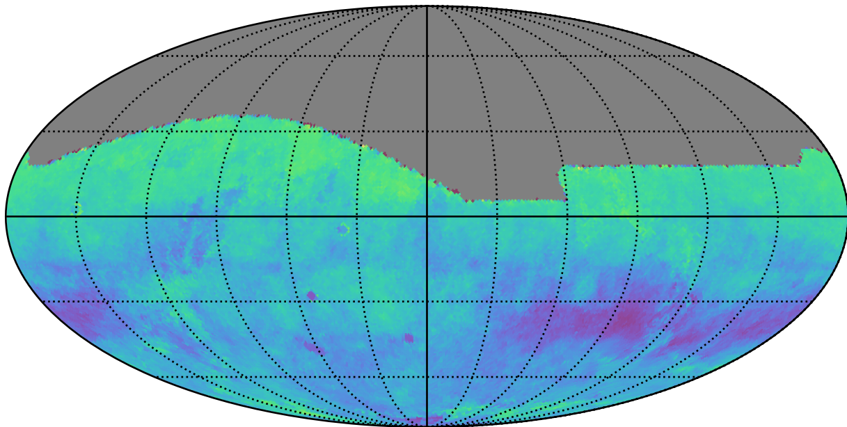
too_elab_r8_d2_ugrizy_v3.4_10yrs r: Kuiper rotSkyPos
