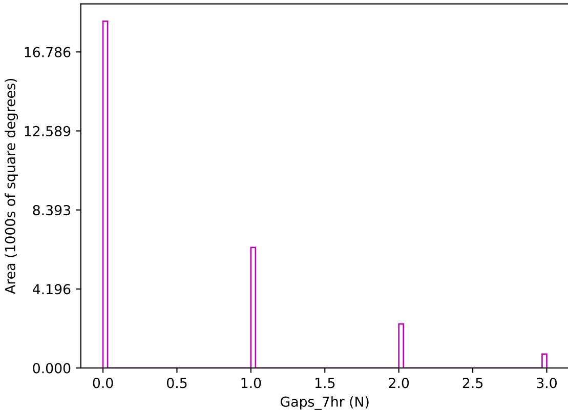
too_elab_r8_d2_ugrizy_v3.4_10yrs z band: Gaps_7hr
