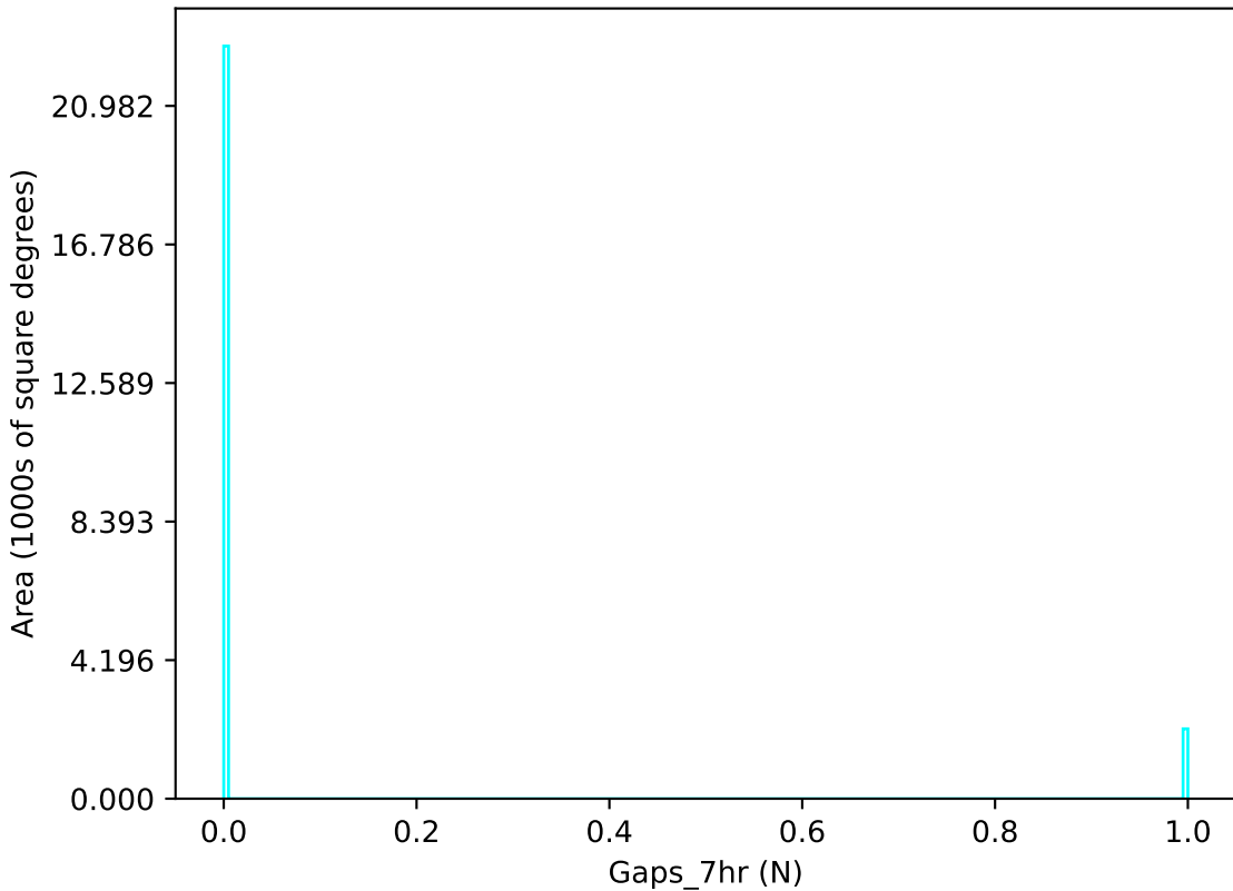
too_elab_r8_d2_ugrizy_v3.4_10yrs u band: Gaps_7hr
