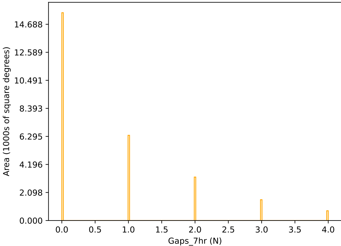
too_elab_r8_d2_ugrizy_v3.4_10yrs r band: Gaps_7hr
