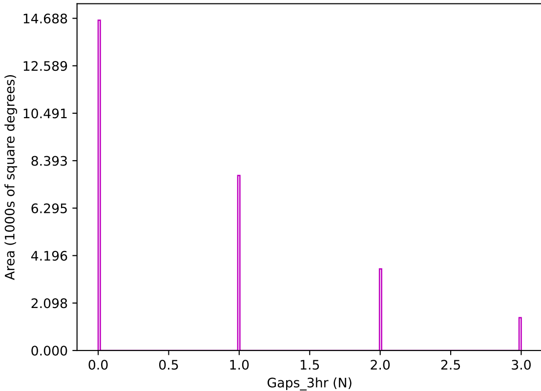
too_elab_r8_d2_ugrizy_v3.4_10yrs z band: Gaps_3hr
