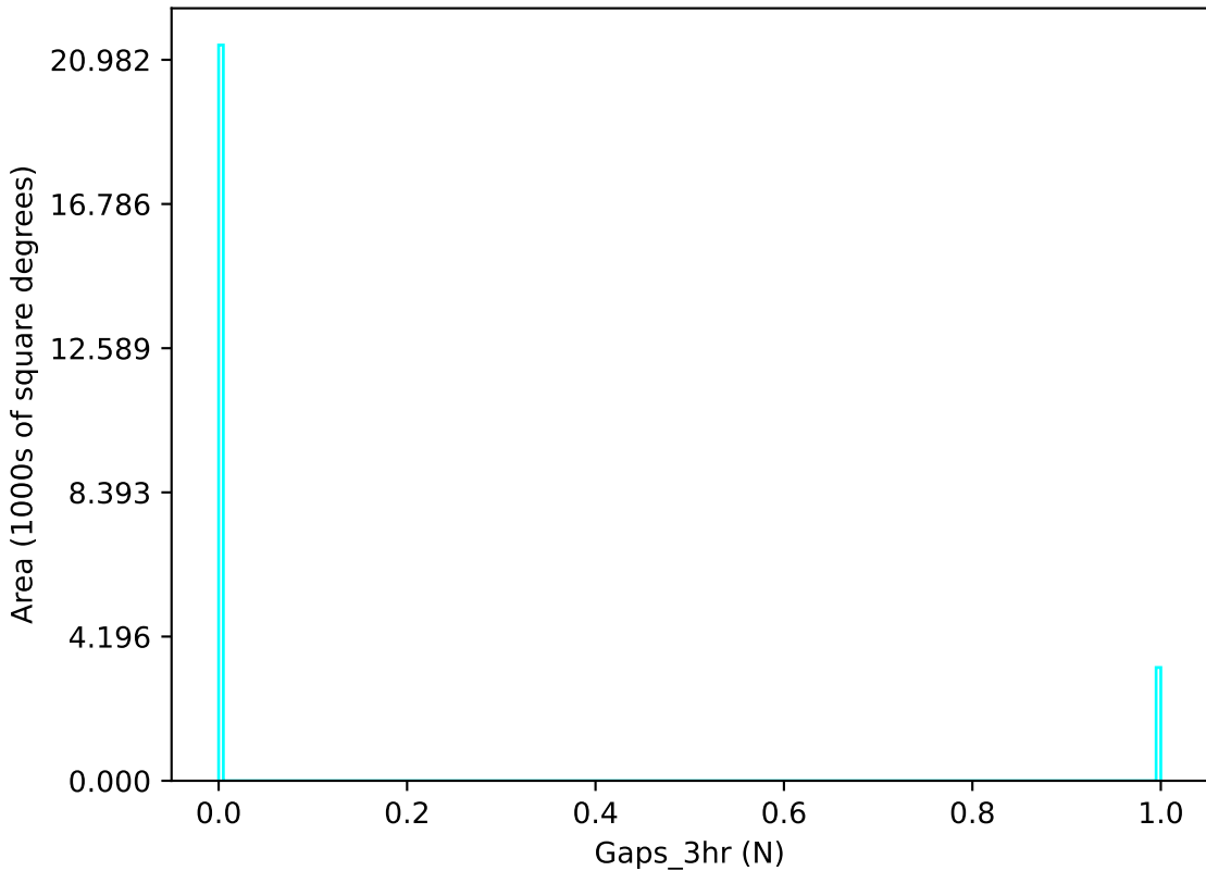
too_elab_r8_d2_ugrizy_v3.4_10yrs u band: Gaps_3hr
