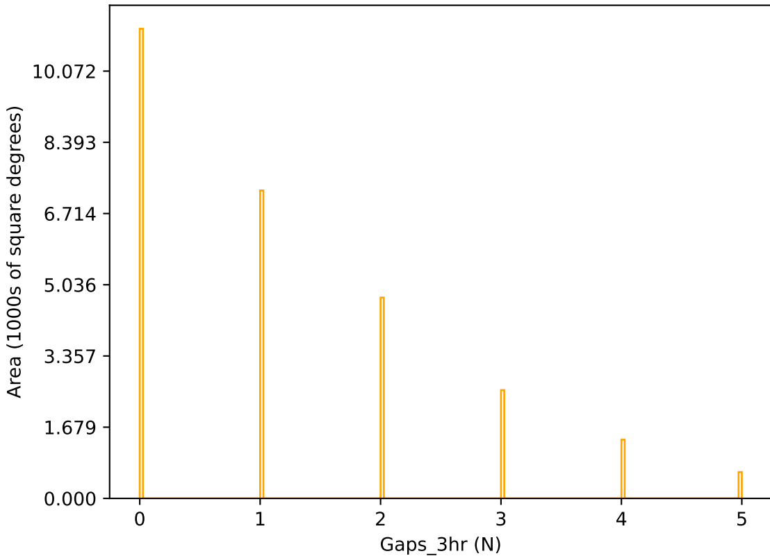
too_elab_r8_d2_ugrizy_v3.4_10yrs r band: Gaps_3hr
