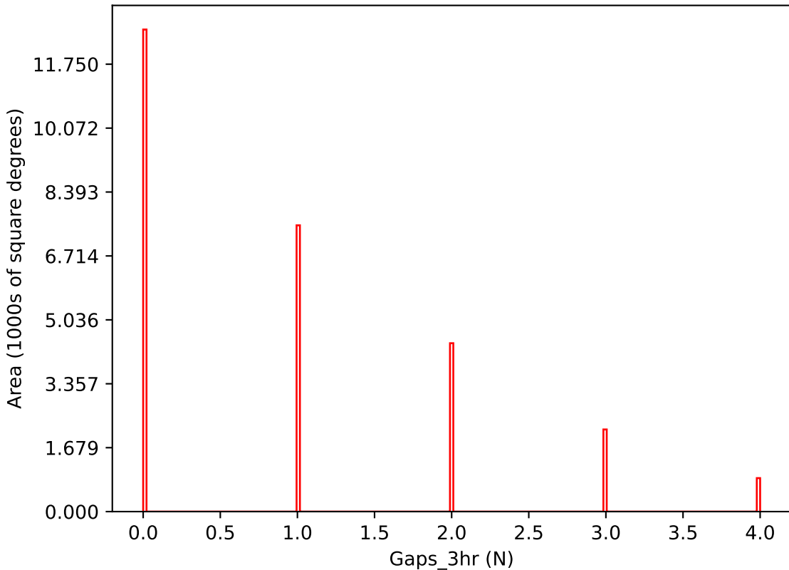
too_elab_r8_d2_ugrizy_v3.4_10yrs i band: Gaps_3hr
