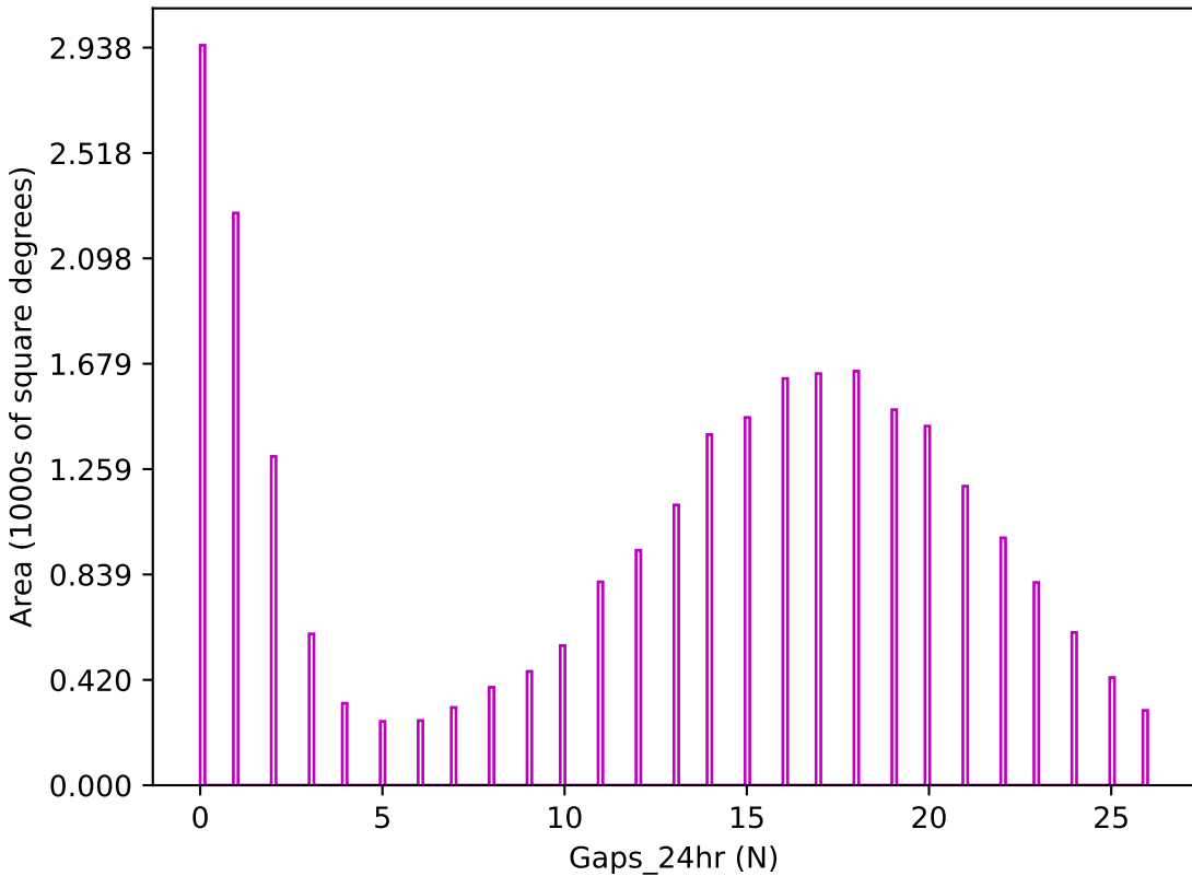
too_elab_r8_d2_ugrizy_v3.4_10yrs z band: Gaps_24hr
