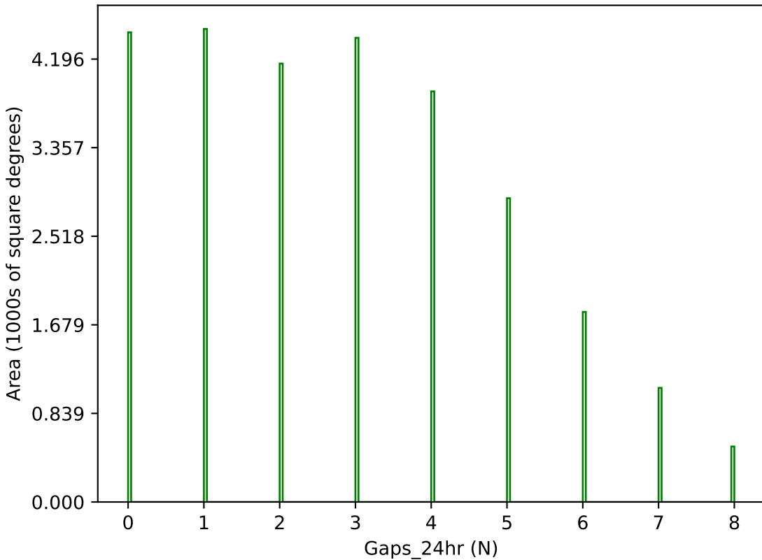
too_elab_r8_d2_ugrizy_v3.4_10yrs g band: Gaps_24hr
