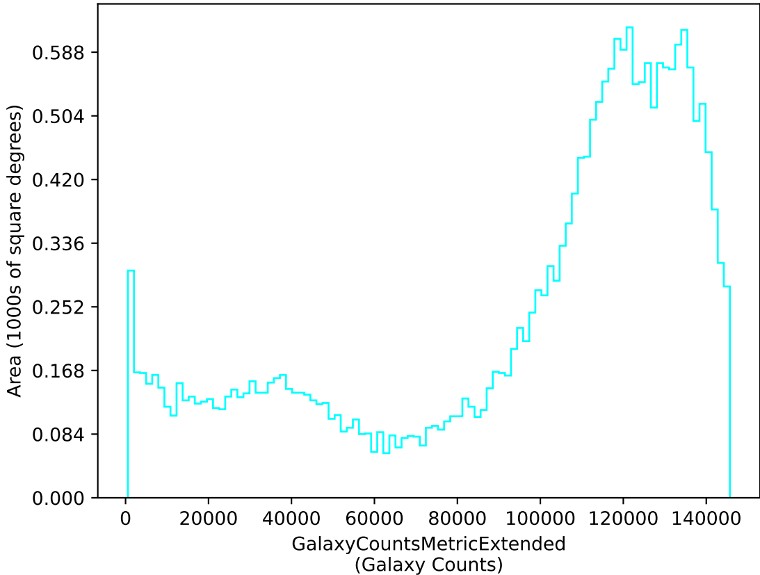
too_elab_r8_d2_ugrizy_v3.4_10yrs u: GalaxyCountsMetricExtended
