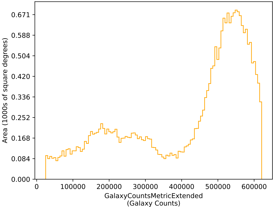
too_elab_r8_d2_ugrizy_v3.4_10yrs r: GalaxyCountsMetricExtended
