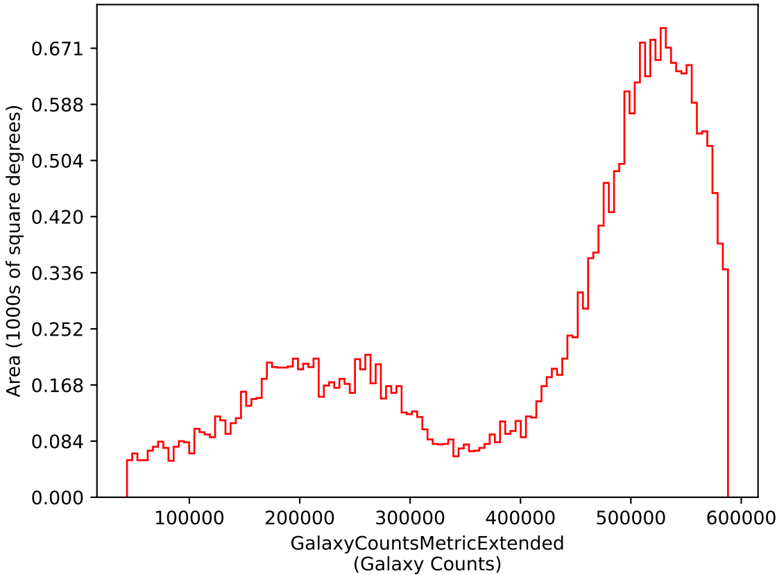
too_elab_r8_d2_ugrizy_v3.4_10yrs i: GalaxyCountsMetricExtended
