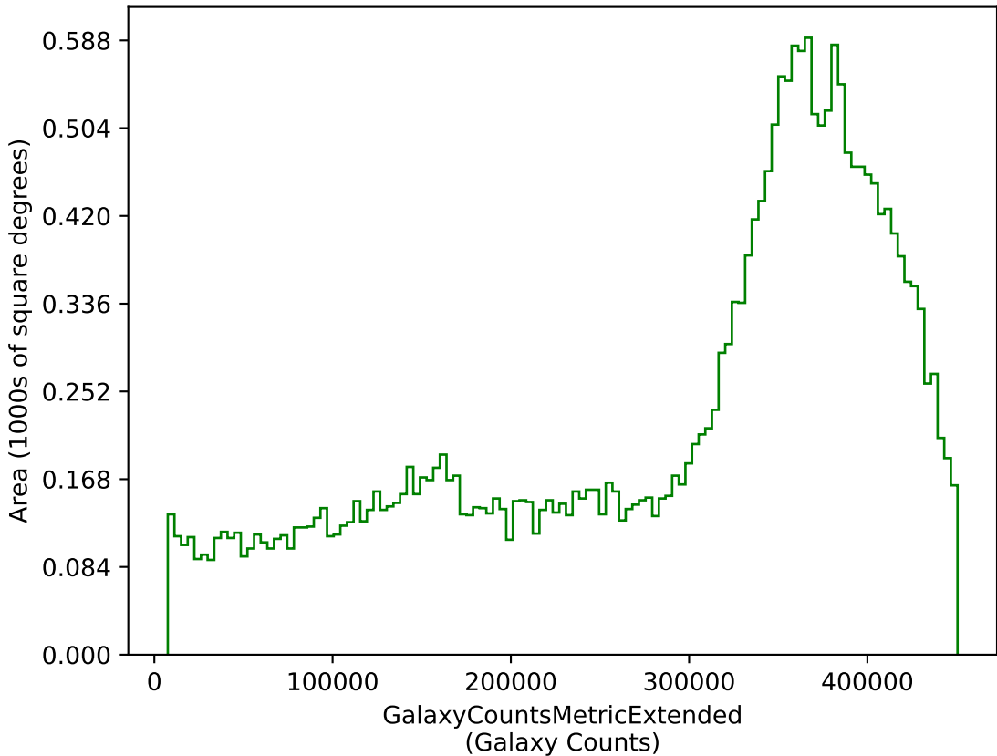
too_elab_r8_d2_ugrizy_v3.4_10yrs g: GalaxyCountsMetricExtended
