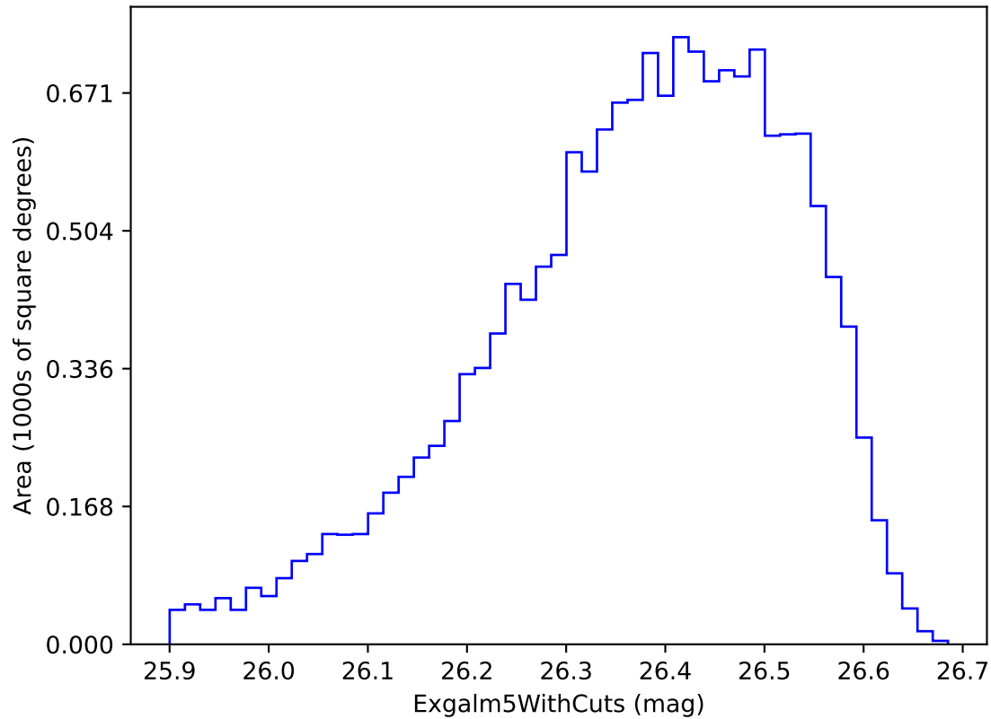
too_elab_r8_d2_ugrizy_v3.4_10yrs i band non-DD year 10: ExgalM5WithCuts
