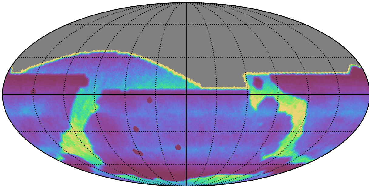
too_elab_r8_d2_ugrizy_v3.4_10yrs : DCRprecision
