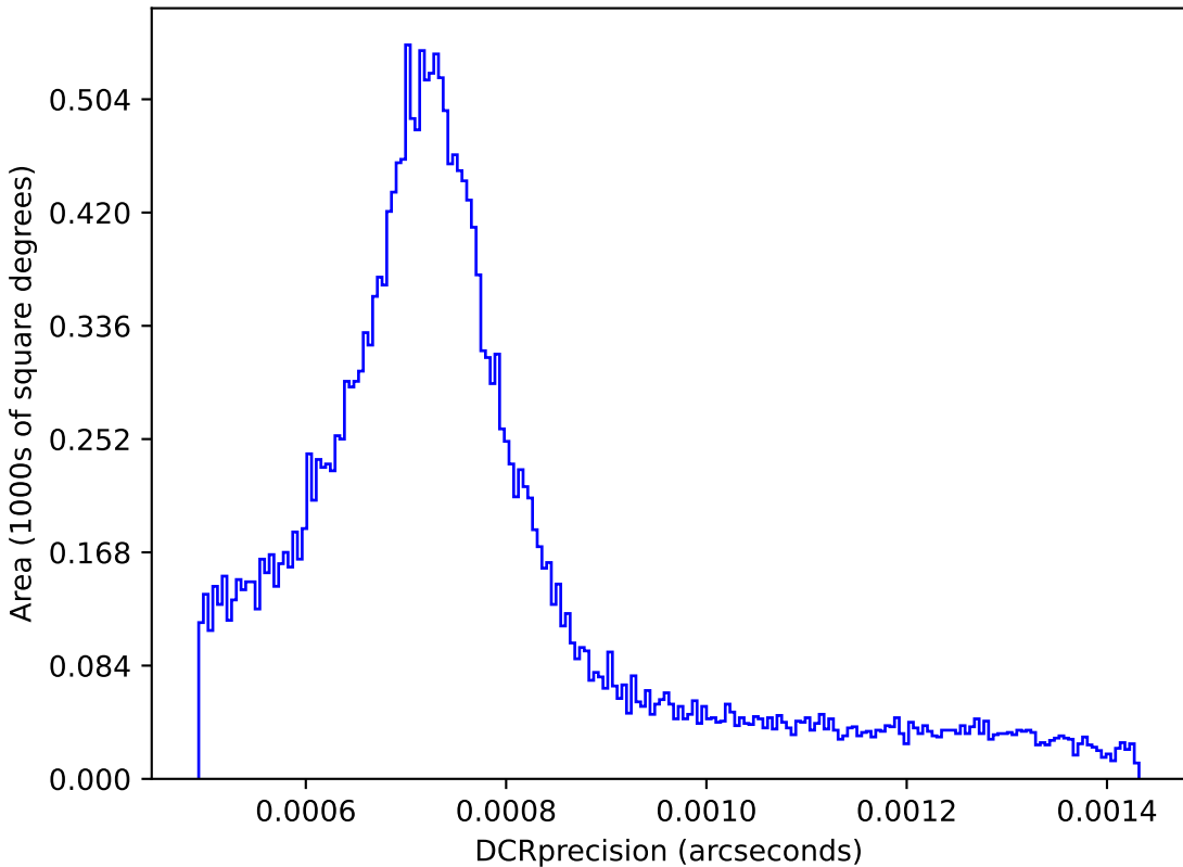
too_elab_r8_d2_ugrizy_v3.4_10yrs : DCRprecision
