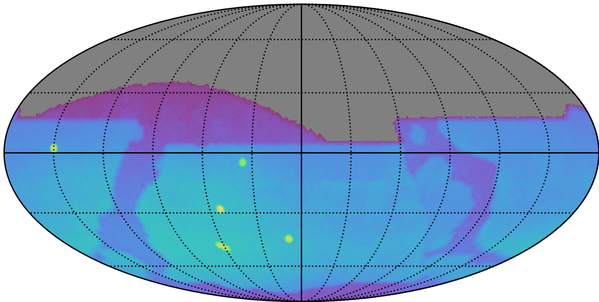
too_elab_r8_d2_ugrizy_v3.4_10yrs : Brown Dwarf, L7
