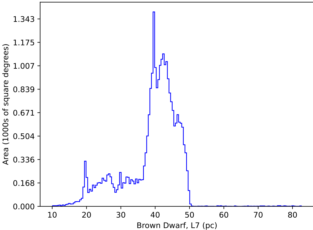
too_elab_r8_d2_ugrizy_v3.4_10yrs : Brown Dwarf, L7
