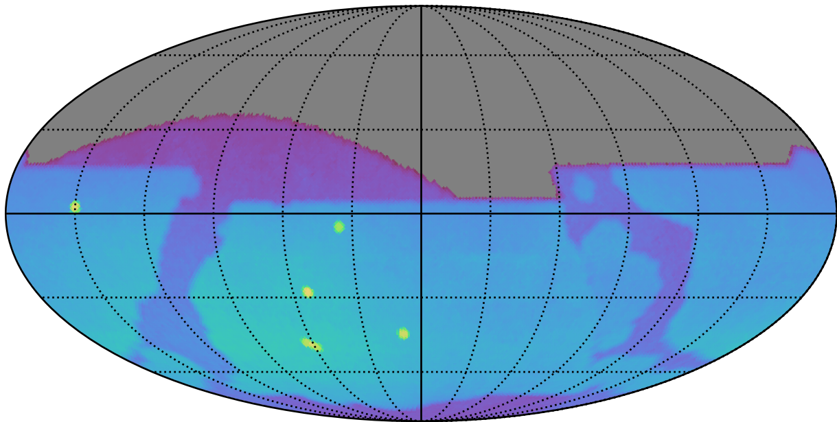
too_elab_r8_d2_ugrizy_v3.4_10yrs : Brown Dwarf, L4
