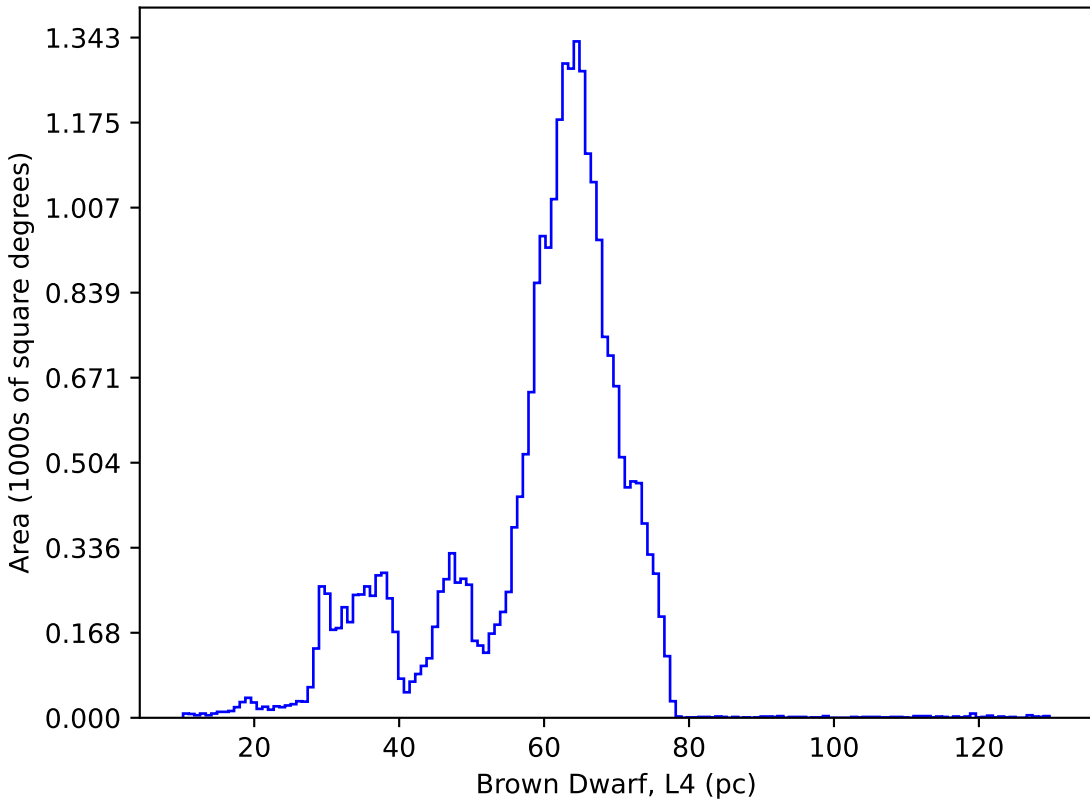
too_elab_r8_d2_ugrizy_v3.4_10yrs : Brown Dwarf, L4
