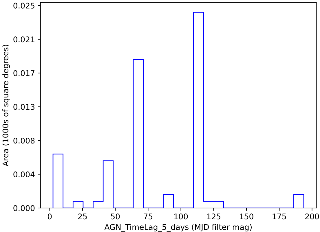
too_elab_r8_d2_ugrizy_v3.4_10yrs y band: AGN_TimeLag_5_days
