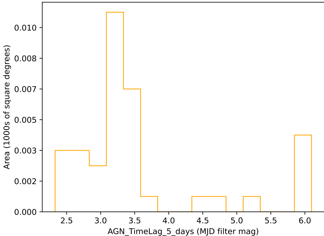
too_elab_r8_d2_ugrizy_v3.4_10yrs r band: AGN_TimeLag_5_days
