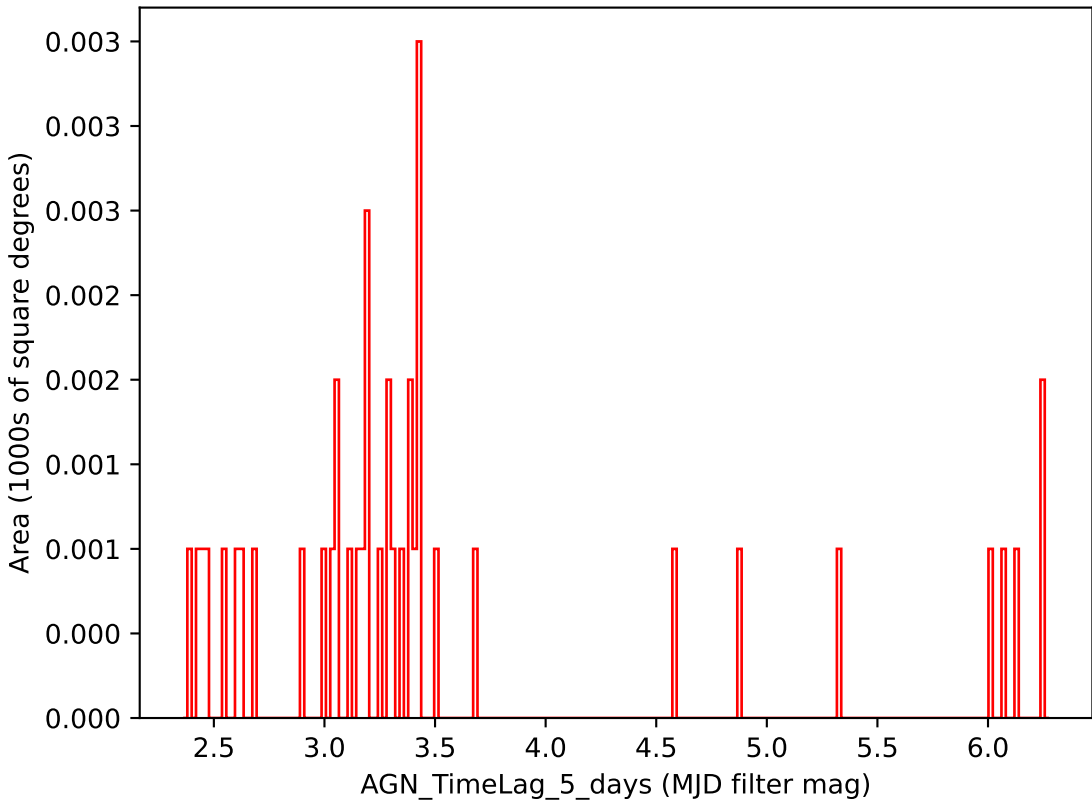
too_elab_r8_d2_ugrizy_v3.4_10yrs i band: AGN_TimeLag_5_days
