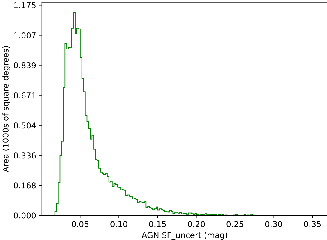
too_elab_r8_d2_ugrizy_v3.4_10yrs g band: AGN SF_uncert
