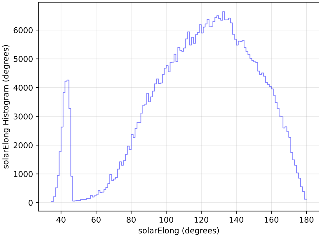
too_elab_r8_d2_ugrizy_v3.4_10yrs WFD z band: solarElong Histogram
