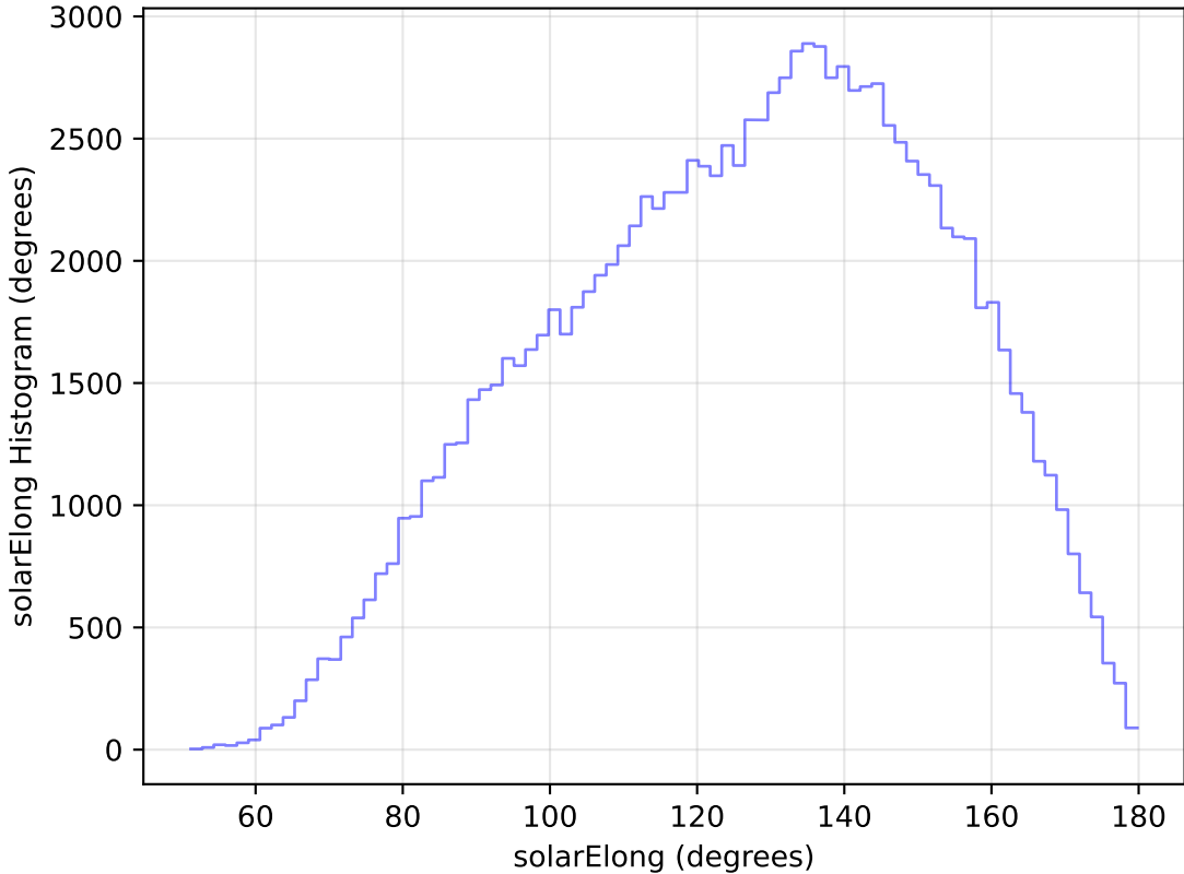
too_elab_r8_d2_ugrizy_v3.4_10yrs WFD u band: solarElong Histogram
