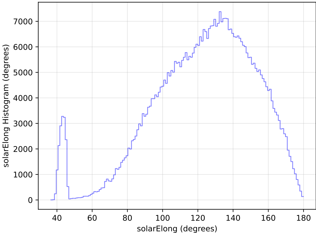
too_elab_r8_d2_ugrizy_v3.4_10yrs WFD r band: solarElong Histogram
