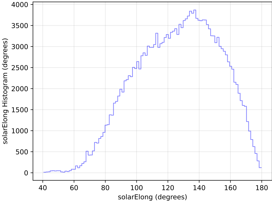
too_elab_r8_d2_ugrizy_v3.4_10yrs WFD g band: solarElong Histogram
