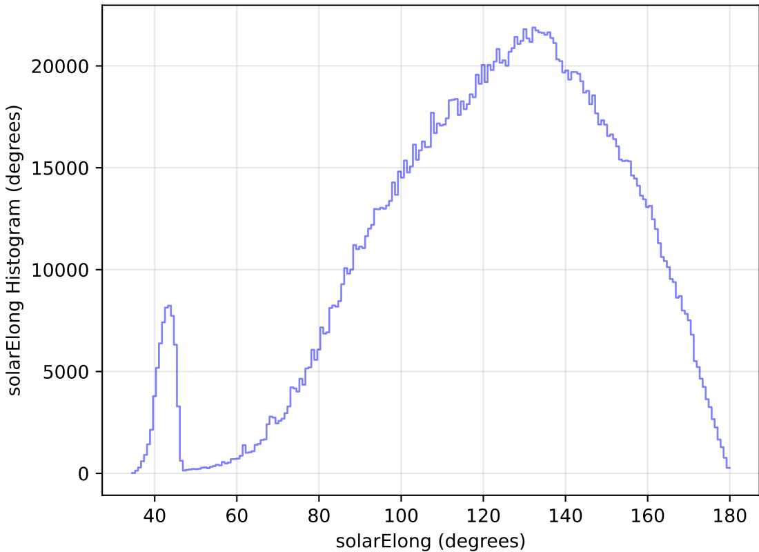
too_elab_r8_d2_ugrizy_v3.4_10yrs WFD all bands: solarElong Histogram
